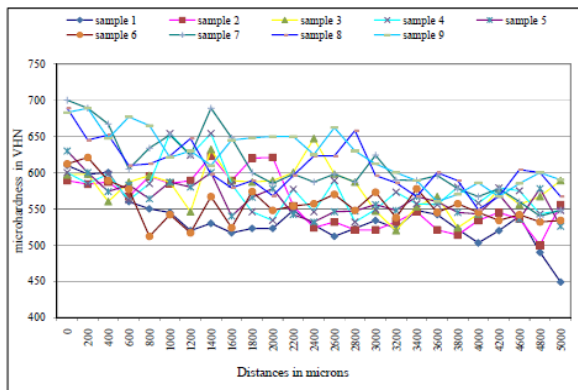
Fig 3: Microhardness profile
